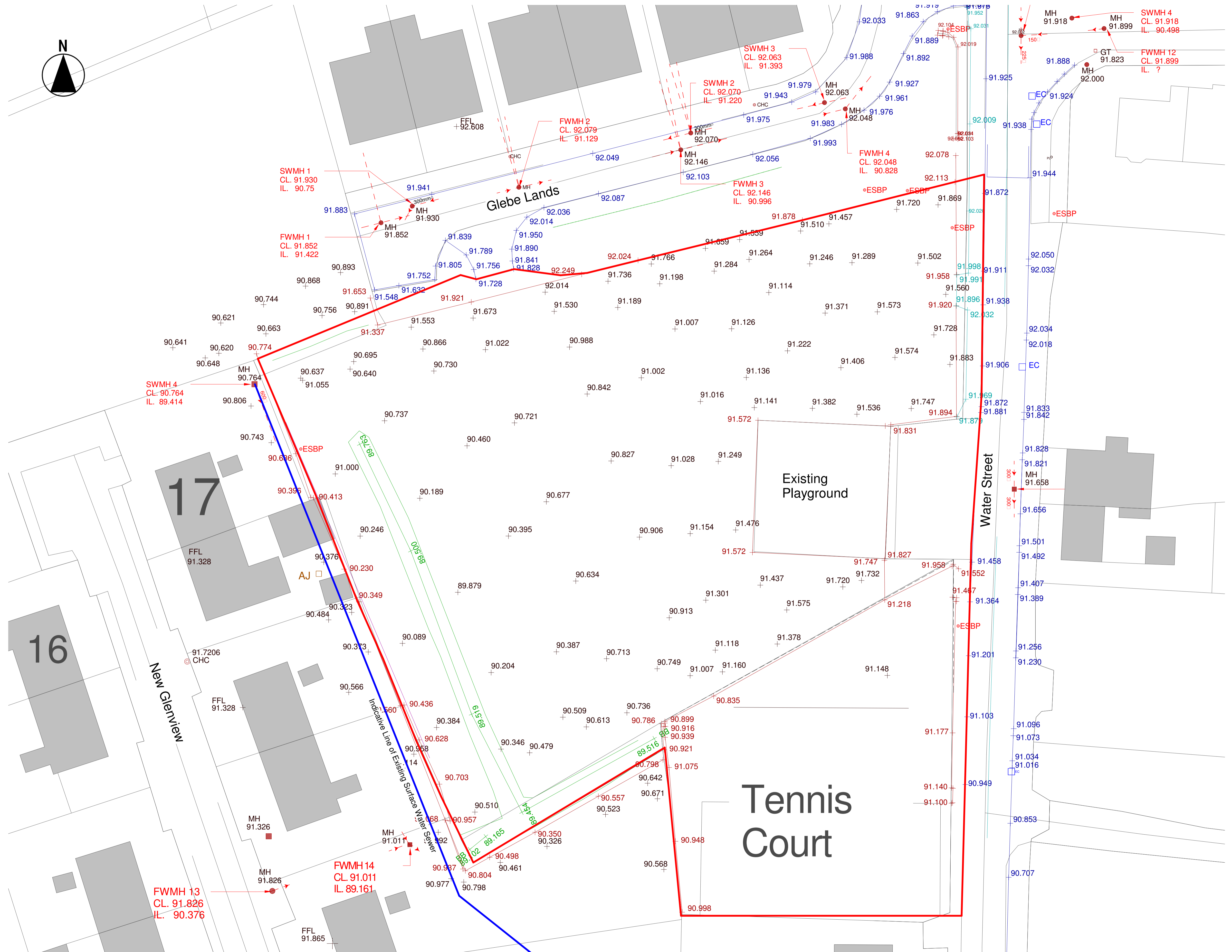
1 Existing Topographic Survey 1 : 250
