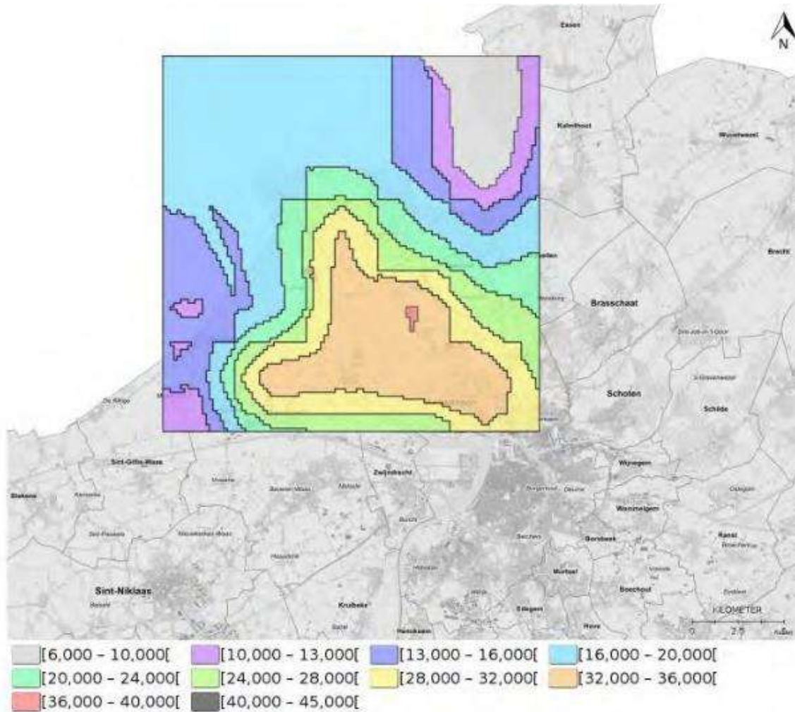
Figure 60: Annual average \text{NO}_2 concentration in \mu\text{g}/\text{m}^3 in planned situation (impact 2026 + background concentrations 2025).
