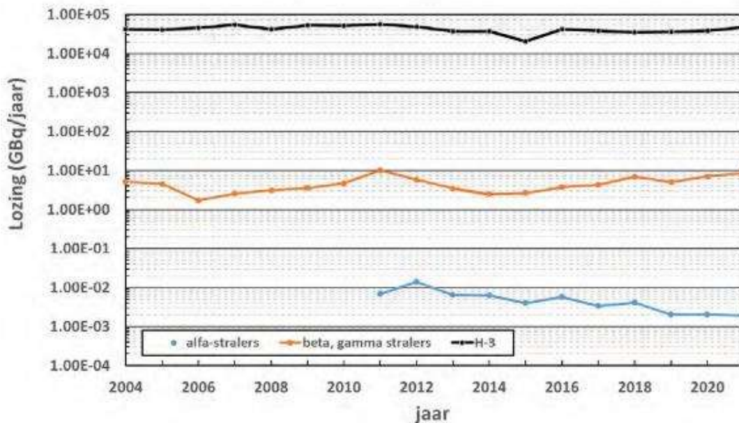
Figure 70: Evolution of liquid discharges from Doel Nuclear Power Plant into the Scheldt for the period 2004-2021. lvii
