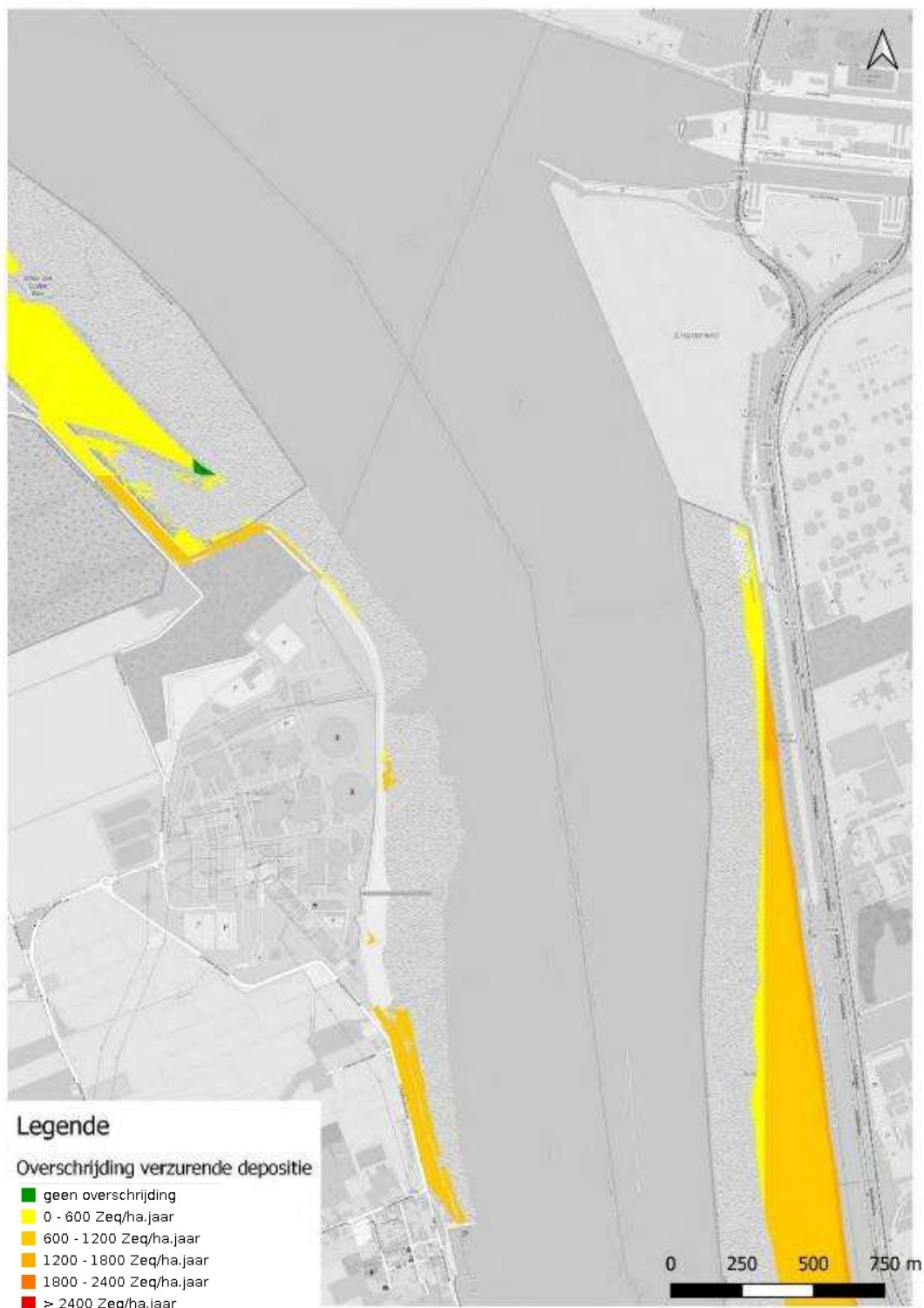
Figure 50: Exceedance map of acidifying deposition.
