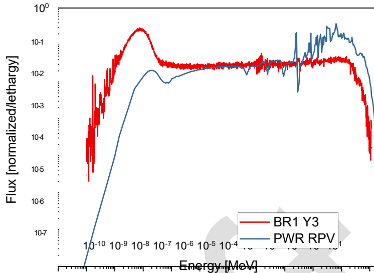
Figure 76: Normalized neutron spectrum per unit of lethargy.
