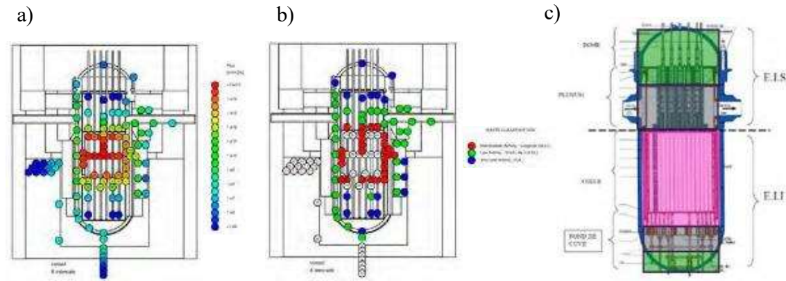
Figure 75: Schematic representation of (a) the simulated neutron flux in a reactor vessel, (b) the waste class classification derived from it, and (c) indication of the transition zone (in gray) for the a priori classification into category A (green) or B waste (purple). a) and b) taken from. lxxvi
