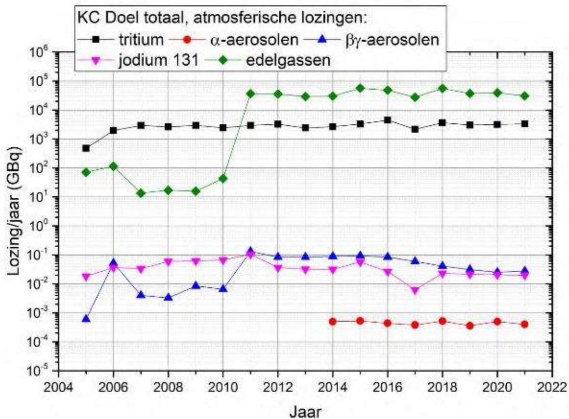
Figure 67: Gaseous discharges per year for the total site of KC Doel 76 .
