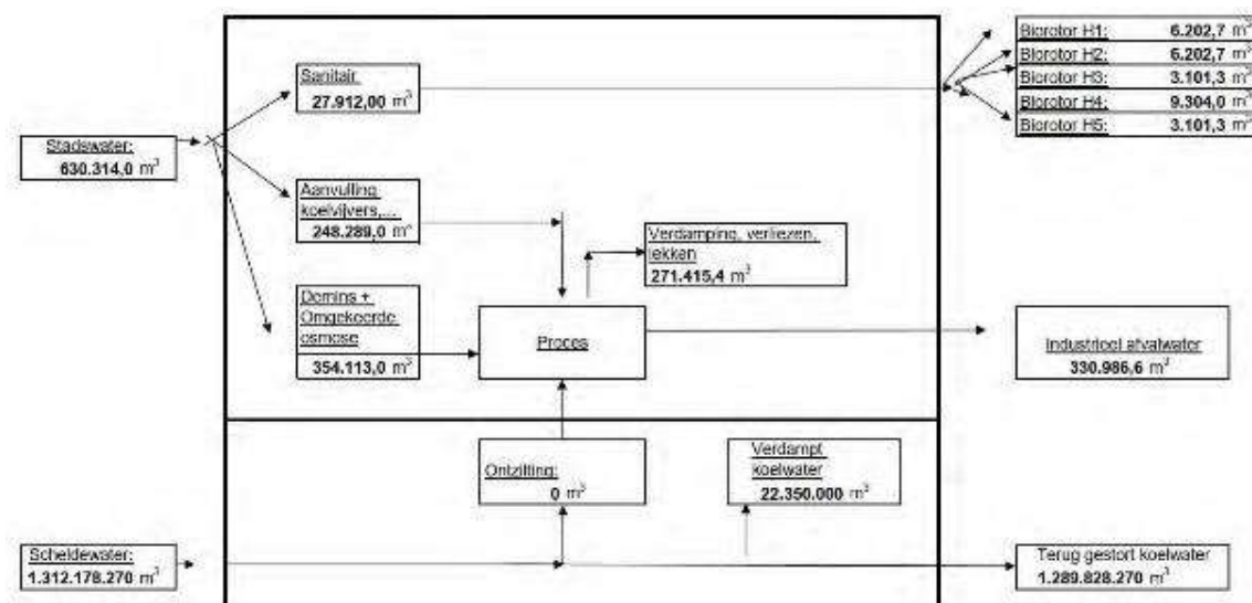
Figure 32: KC Doel water balance for 2021.
