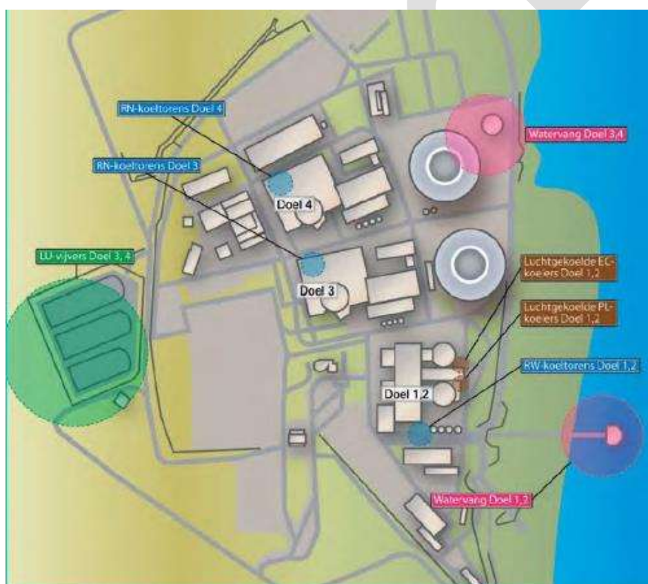
Figure 44: Cooling water principle diagram showing water capture Doel 1&2 and Doel 3&4 (Source: Electrabel nv, 2011).
