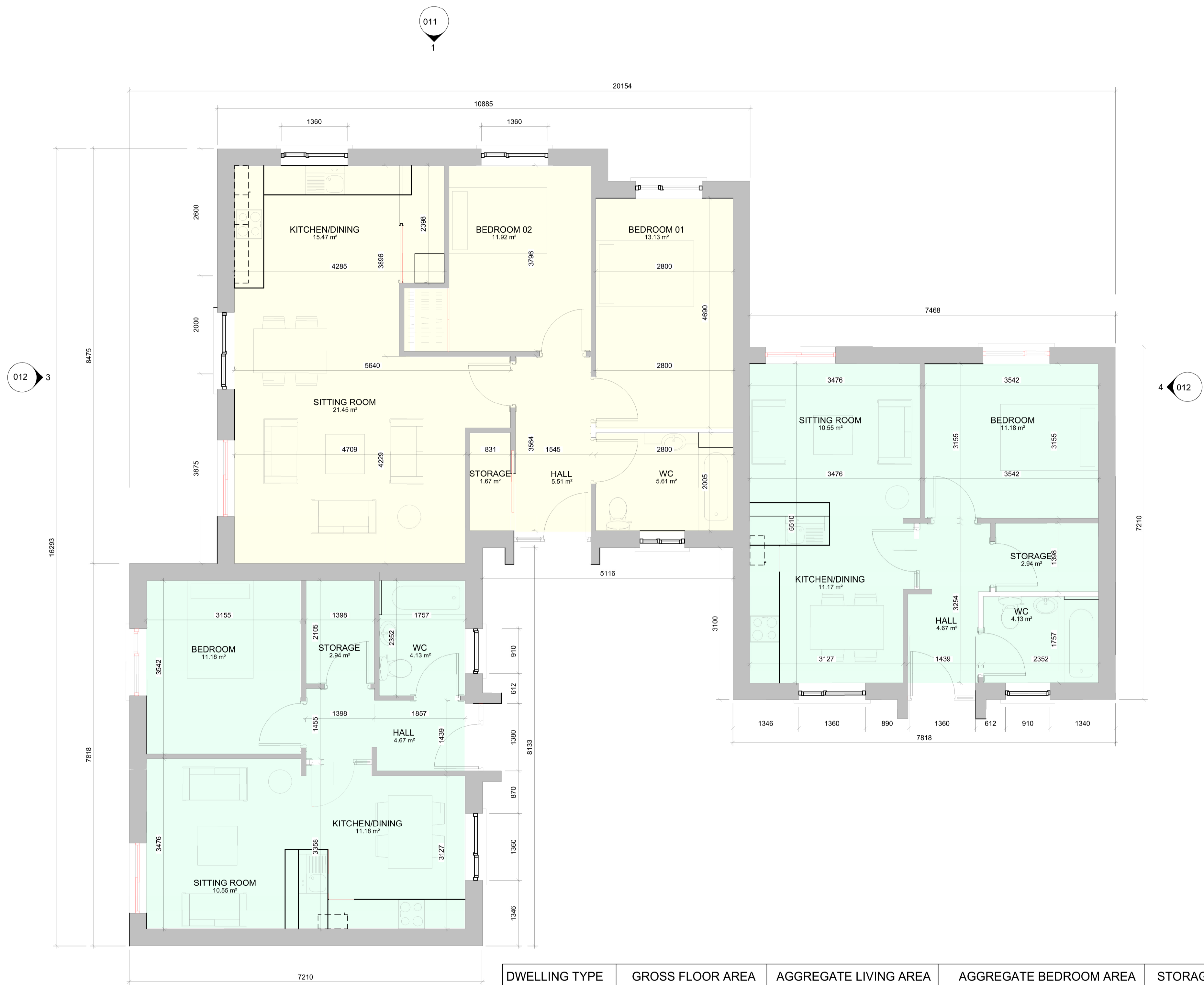
1 Ground Floor Level 1 : 50
