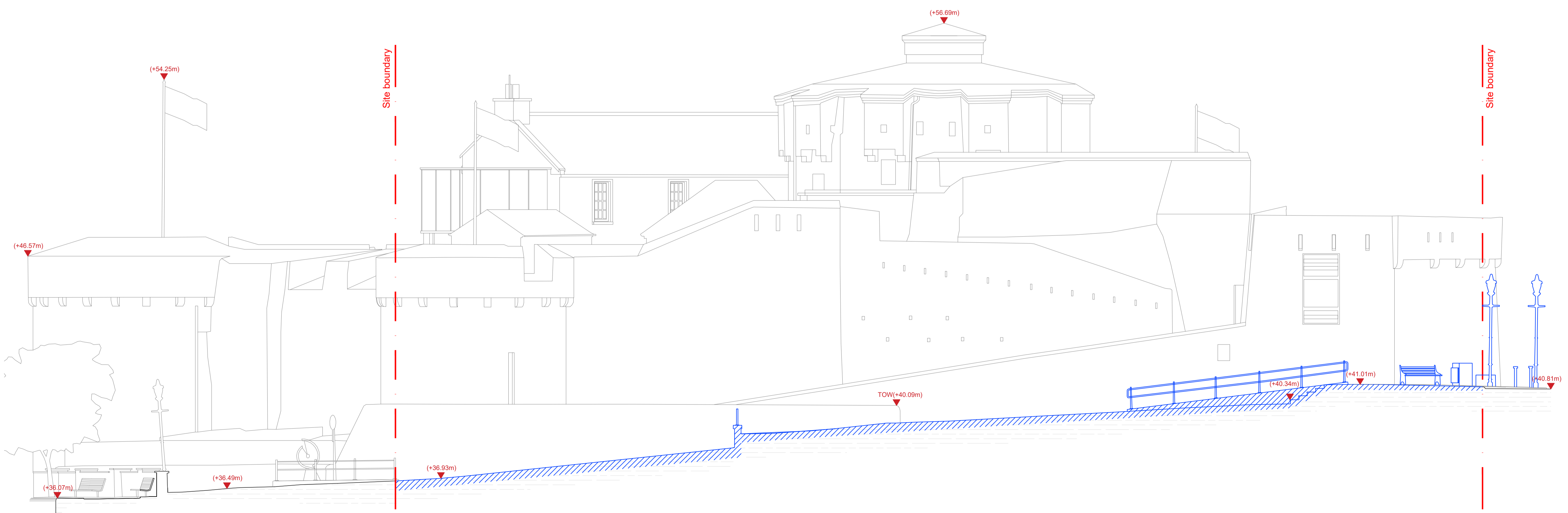
3 EXISTING SECTIONAL ELEVATION C-C 1:100 @ A1
